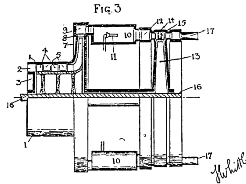
The W.1 turbojet engine
